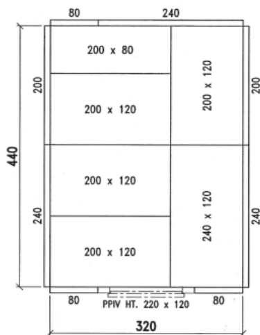
Layout of panels
